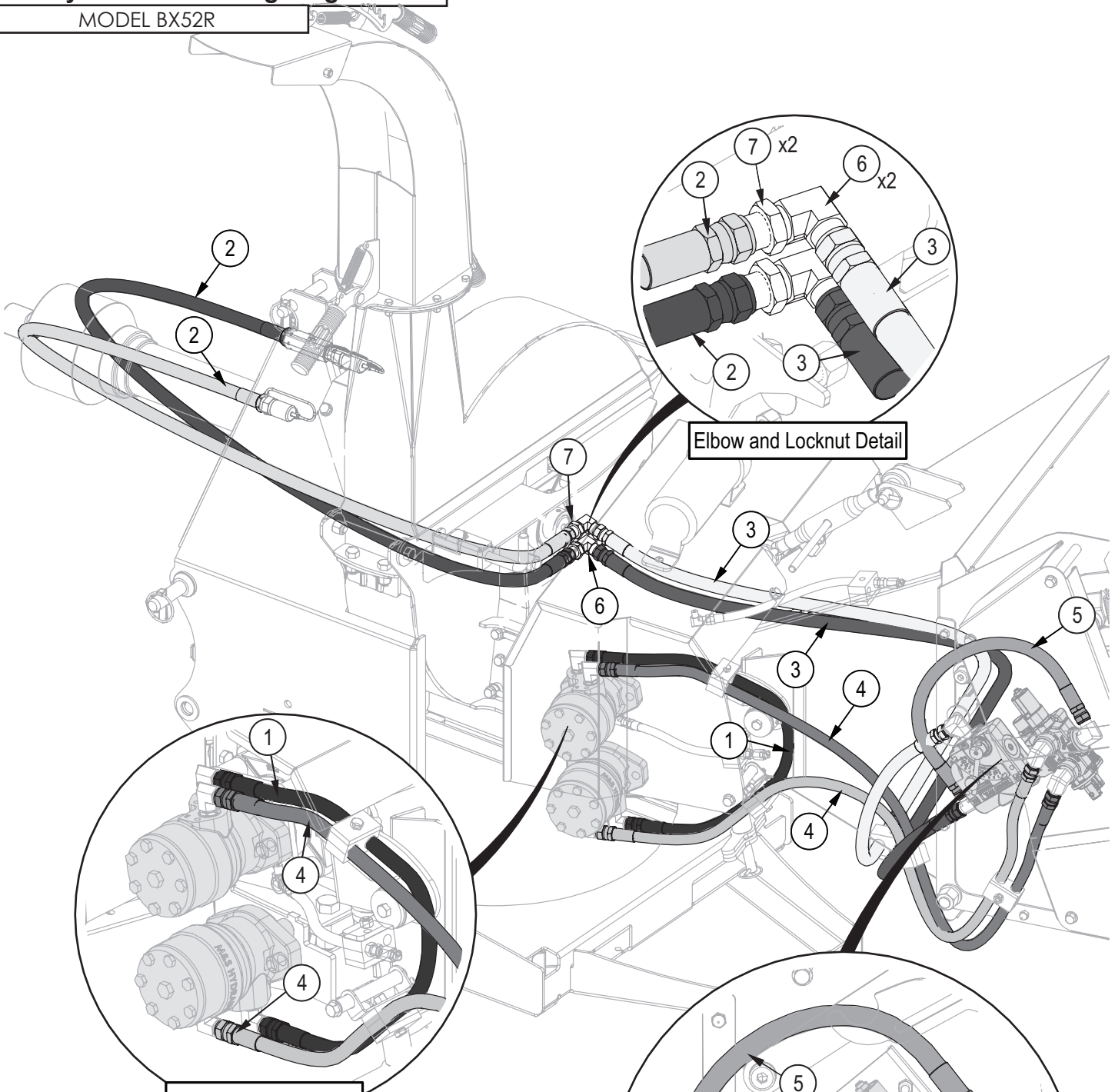
Motor Assembly Detail
