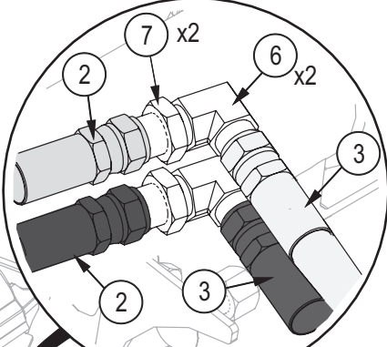
Elbow and Locknut Detail
