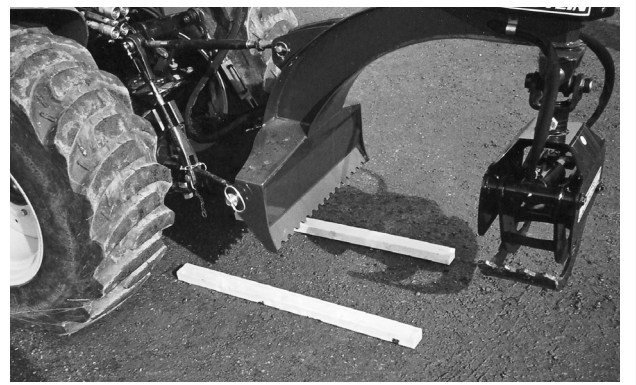
Fig. 11 LEVELLING ADJUSTMENTS
