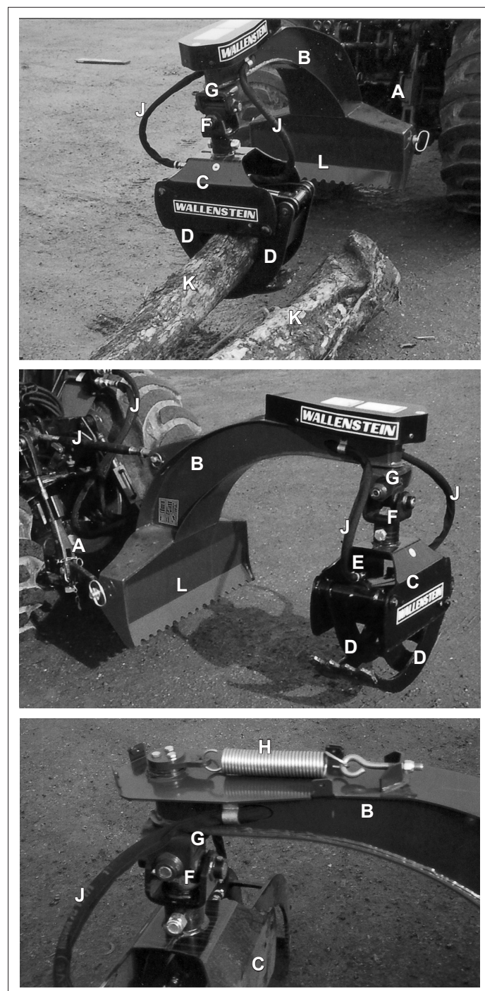
Fig. 1 MACHINE COMPONENTS
